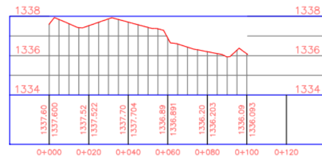
X-X PROFILE
