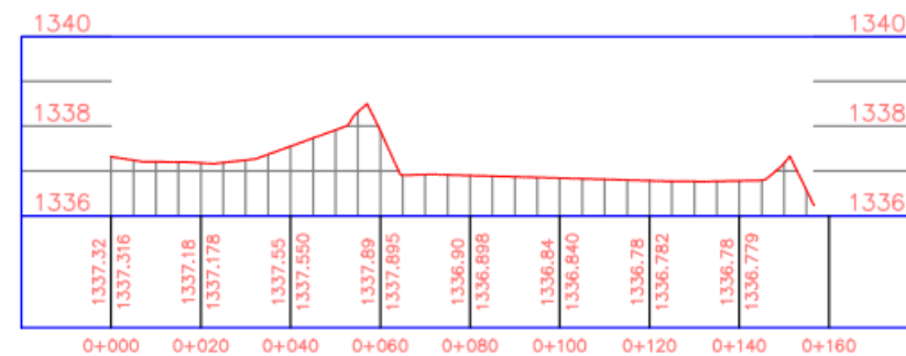
X-X PROFILE
